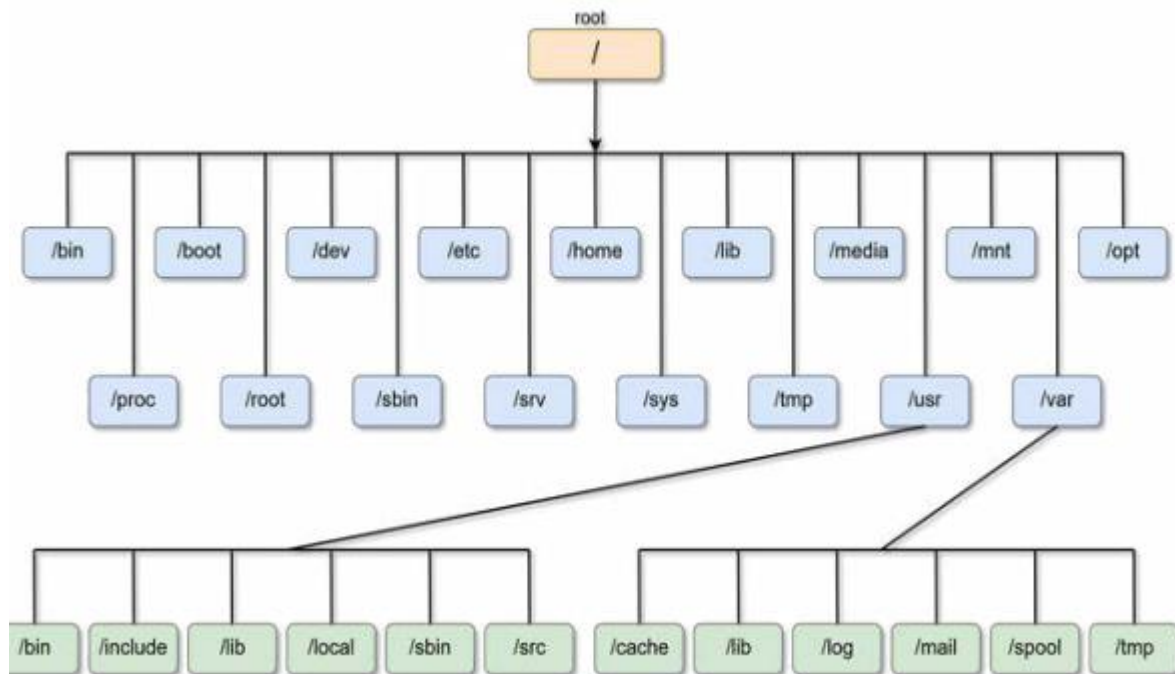
Linux File System
